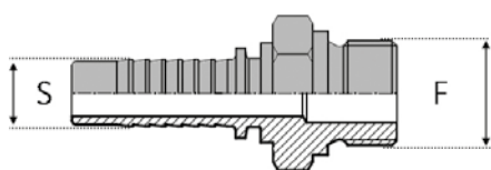
Filetage Whitworth
