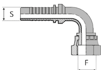
Filetage Whitworth
